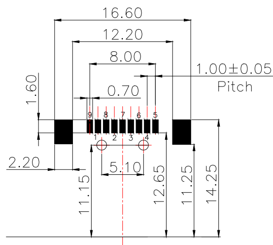
PCB EDGE RECOMMENDED PCB LAYOUT
