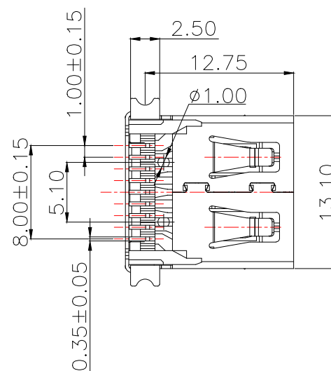
PCB EDGE RECOMMENDED PCB LAYOUT
