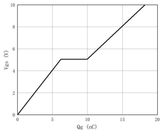
Figure 4. Gate-Charge Characteristics
