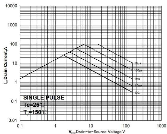
Figure 13. Safe Operating Area
