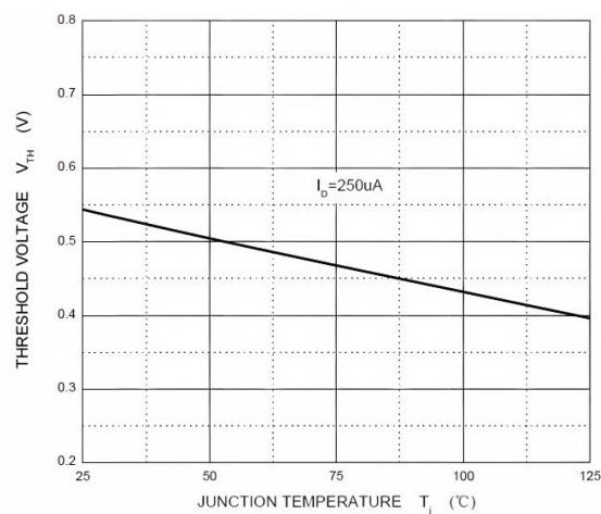
Figure 6. Threshold Voltage
