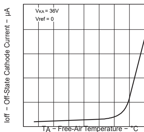
Figure 5. Off-State Cathode Current vs Free-Air Temperature
