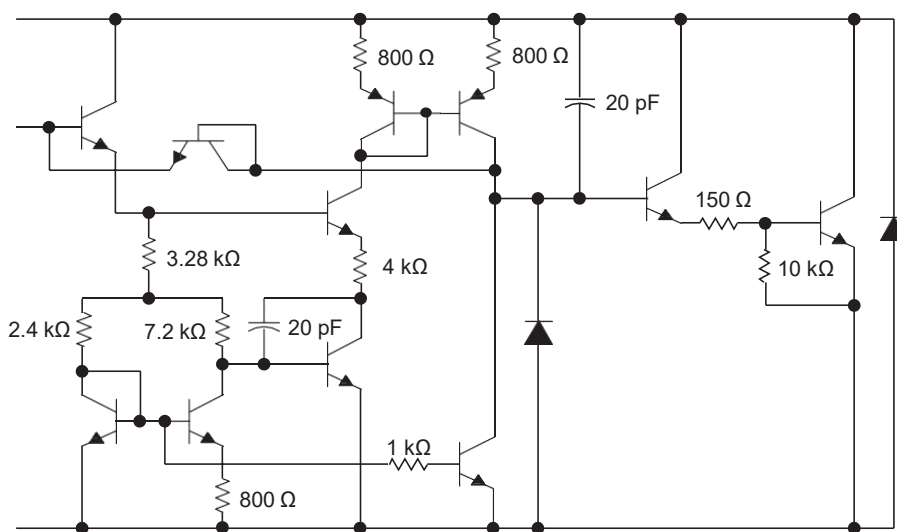
Figure 24. Detailed Schematic
