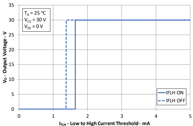
Figure 6: I_{FLH} Hysteresis
