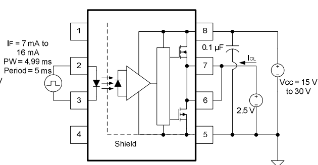
Figure 15 : V_{OL} Test Circuit
