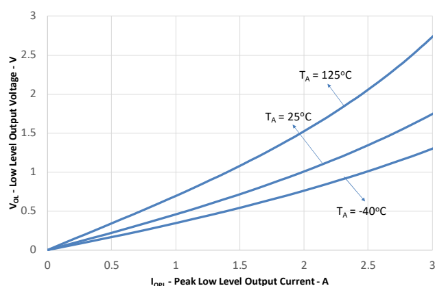
Figure 12: V_{OL} vs. I_{OPL}
