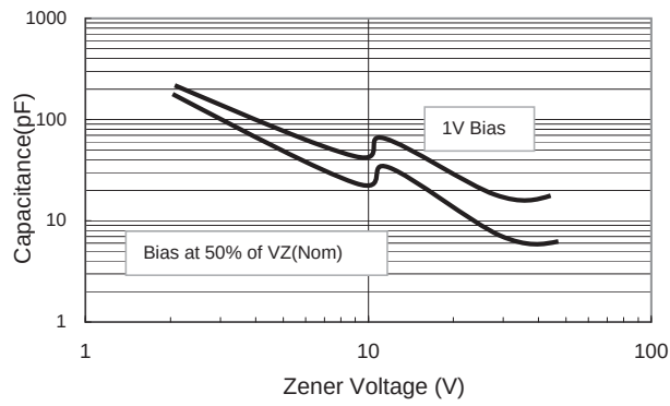
FIG 5 Typical Capacitance
