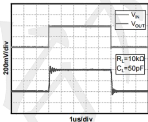
Figure 6. Small-Signal Step Response( V_S=5V )
