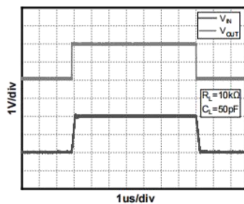
Figure 7. Large-Signal Step Response( V_S=5V )
