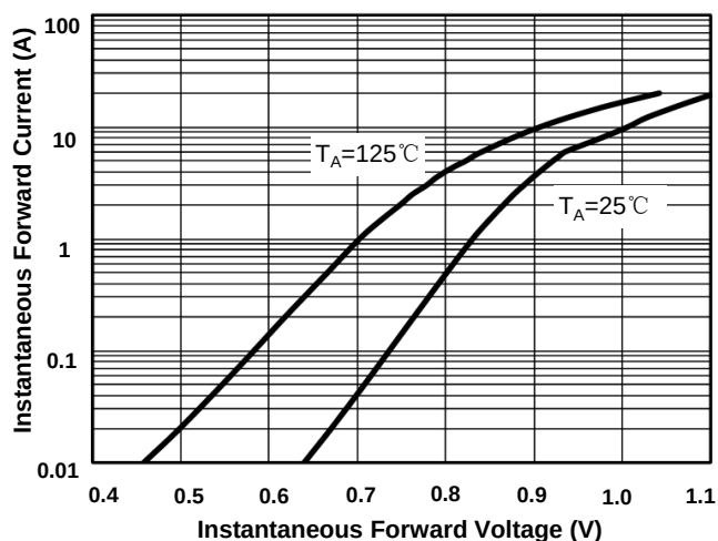
FIG.2-TYPICAL FORWARD CHARACTERISTICS PER DIODE
