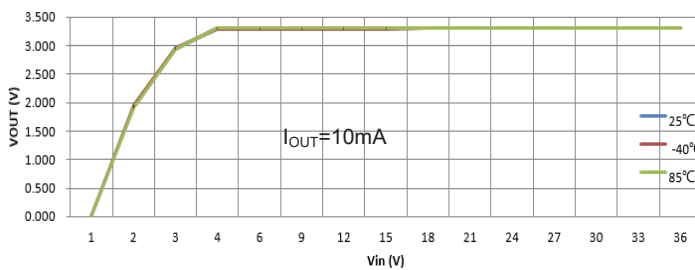
Line Regulation
