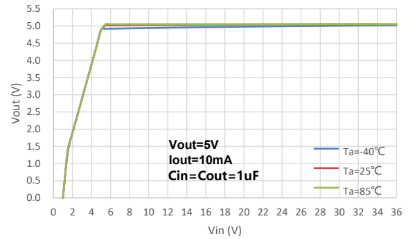
Line Regulation
