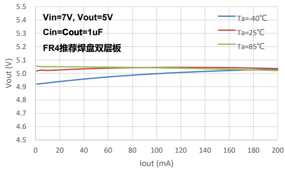
Load Regulation
