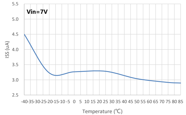
Ground Current vs. Temperature
