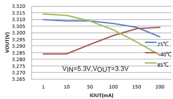
Load Regulation
