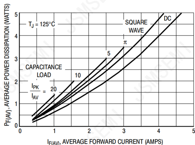
Figure 6. Power Dissipation
