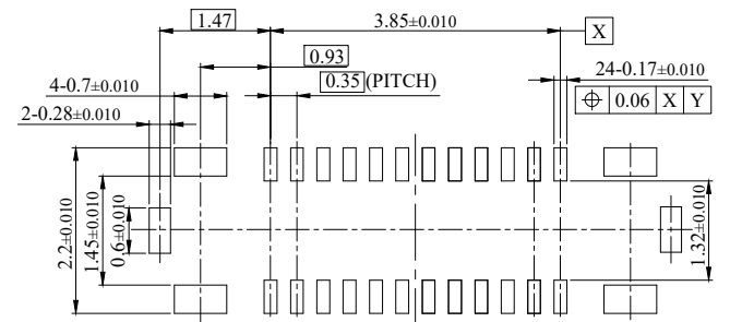
RECOMMENDED METAL DIMENSIONS (THICKNESS: 0.08 mm)
