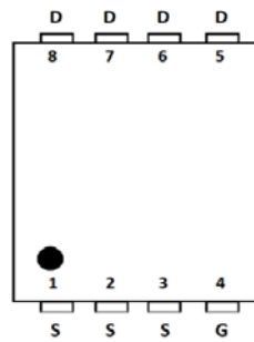
Pin Assignment
