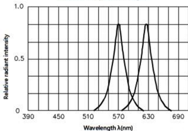
光谱分布曲线 Relative Intensity Vs. Wavelength
