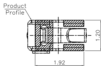
RECOMMENDED PCB LAYOUT TOLERANCE±0.05(焊盘推荐图) (FOR REFERENCE ONLY)
