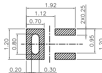
RECOMMENDED METAL MASK TOLERANCE±0.08(钢网推荐图) (FOR REFERENCE ONLY)
