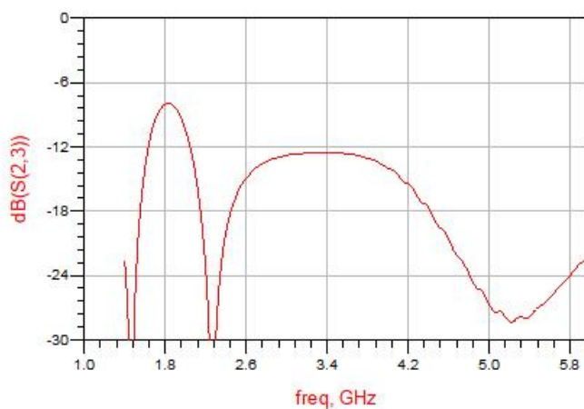
Common Isolation
