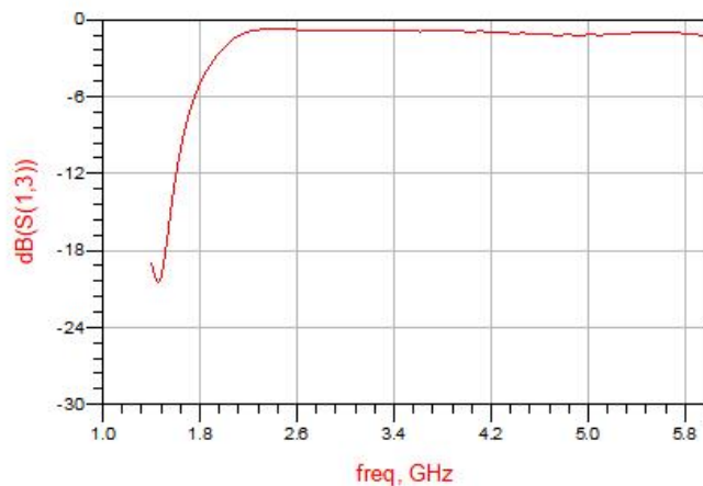
High-Band Attenuation
