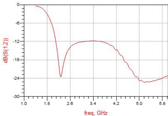
Low-Band Attenuation
