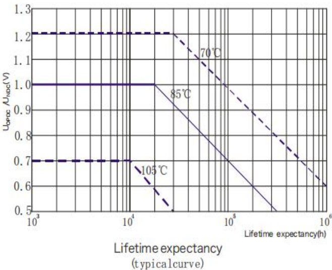
预计寿命曲线 (Lifetime expectancy curve)
