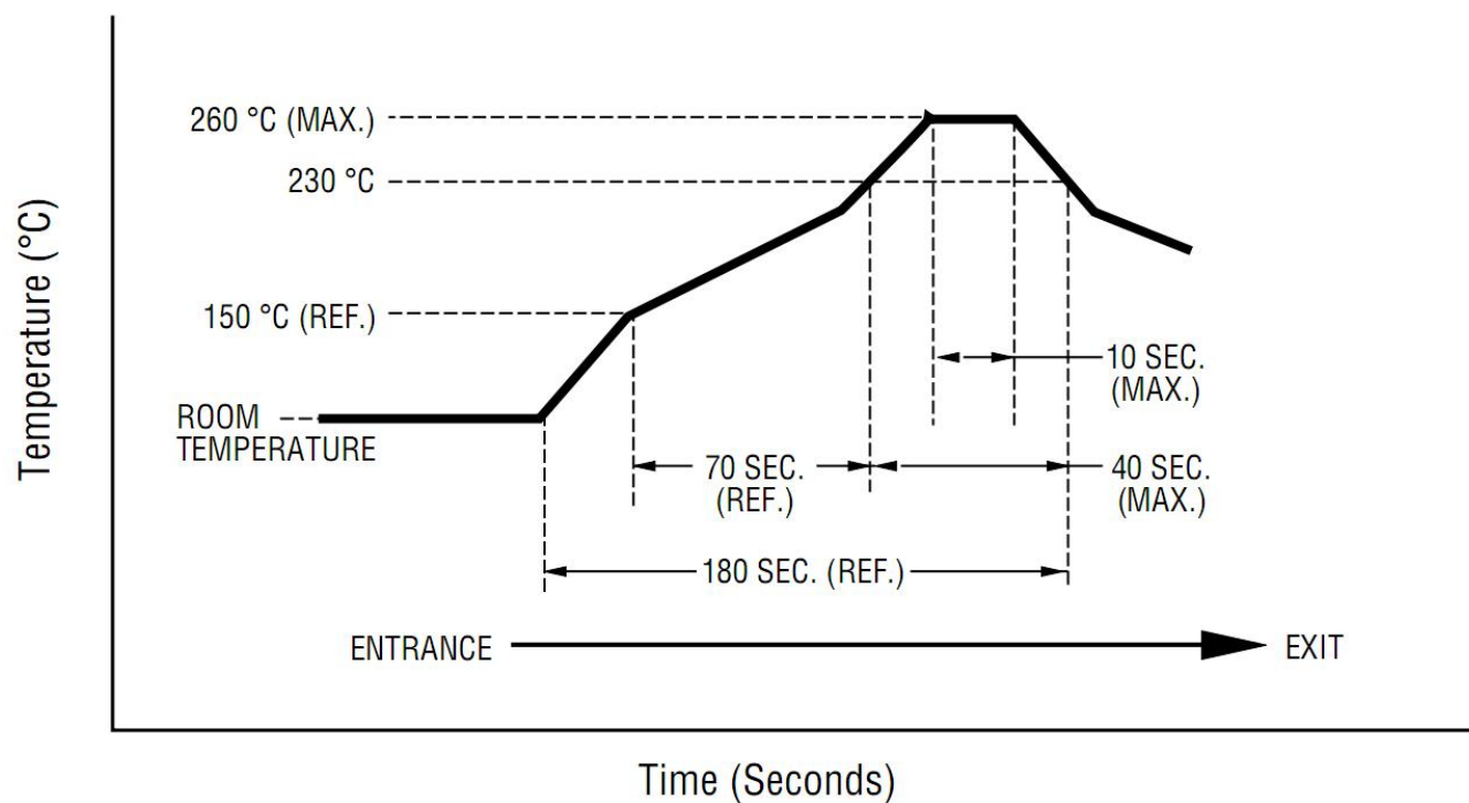
Figure 12. MHC58S03 Thermal Reflow Profile
