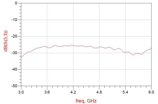
Figure 6. MHC58S03 Return Loss (S33)
