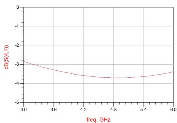
Figure 4. MHC58S03 Transmission
