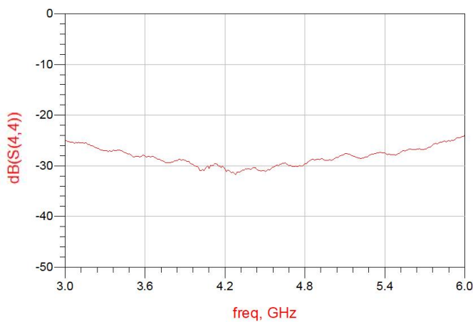
Figure 7. MHC58S03 Return Loss (S44)
