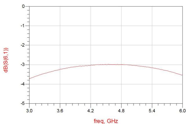
Figure 3. MHC58S03 Coupling
