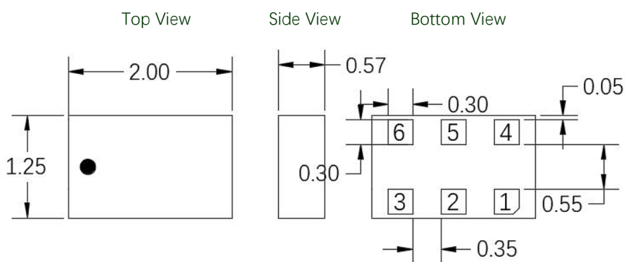
Figure 2. MHC58S03 Outline Drawing
