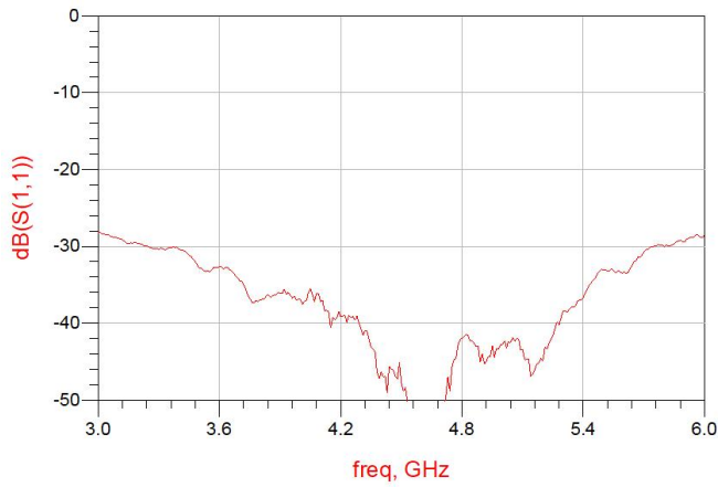
Figure 5. MHC58S03 Return Loss (S11)
