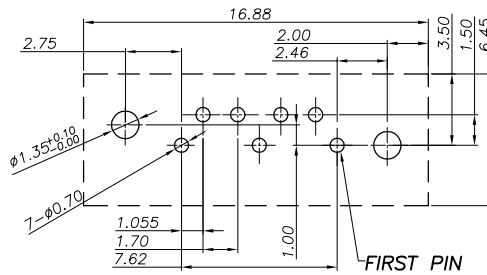
P.C.B LAYOUT(TOP VIEW) TOLERANCE:±0.05
