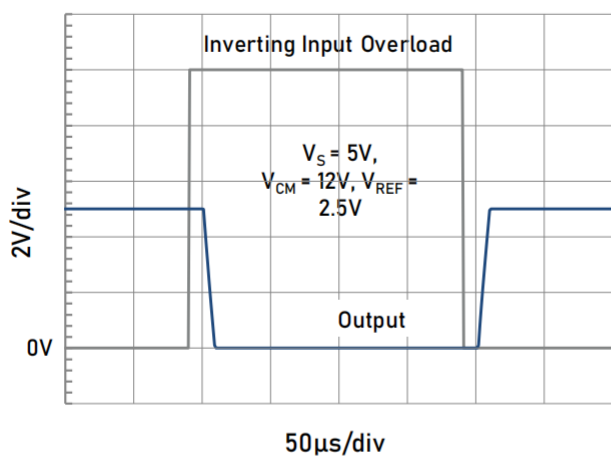
Inverting Differential Input Overload
