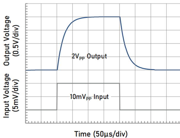
Step Response (10mV pp Input Step)
