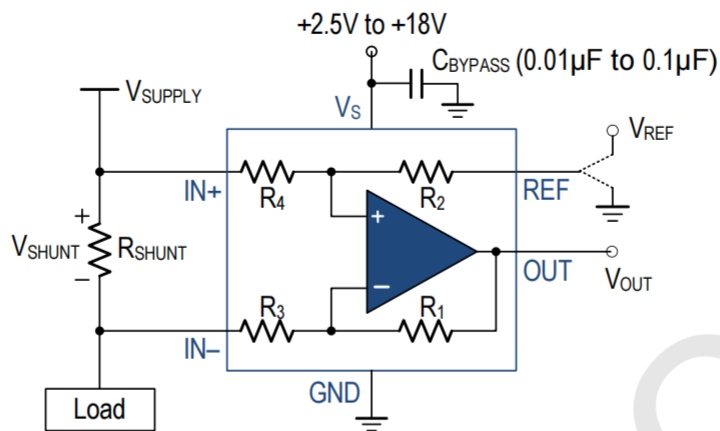
High-side Sensing Application
