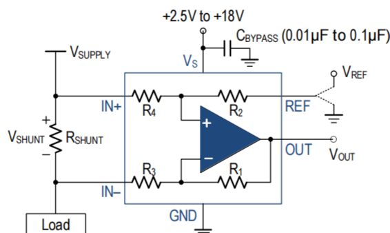
High-side Sensing Application Figure 1. Typical Application
