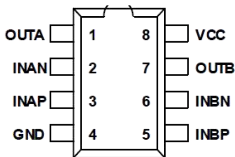
SOP-8/DIP-8
