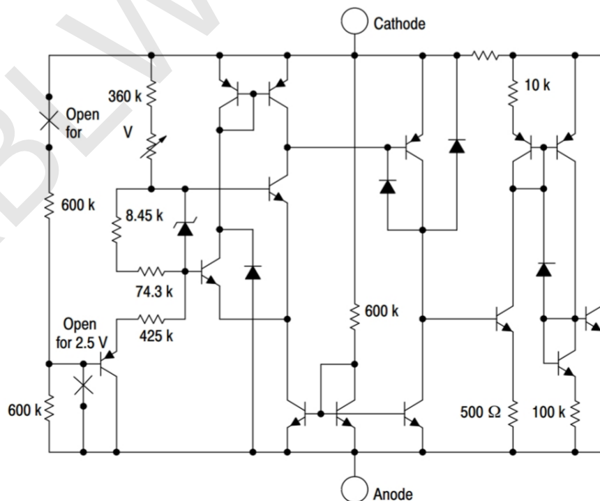
Figure1 Function Block Diagram of LM385
