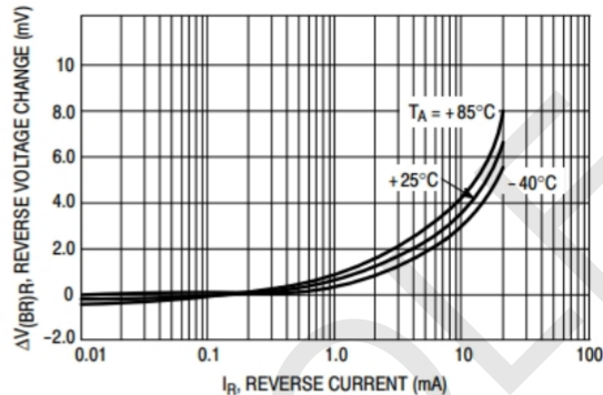
Reverse Characteristics
