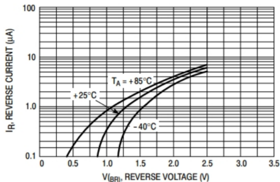
Reverse Characteristics
