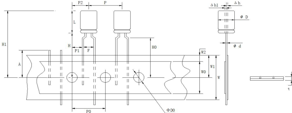
[ Fig. 1 (Diameter for Φ4 to Φ8)]
