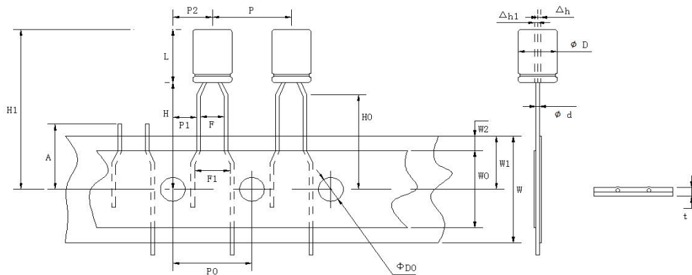
[ Fig. 2 (Diameter for Φ4 to Φ5)]
