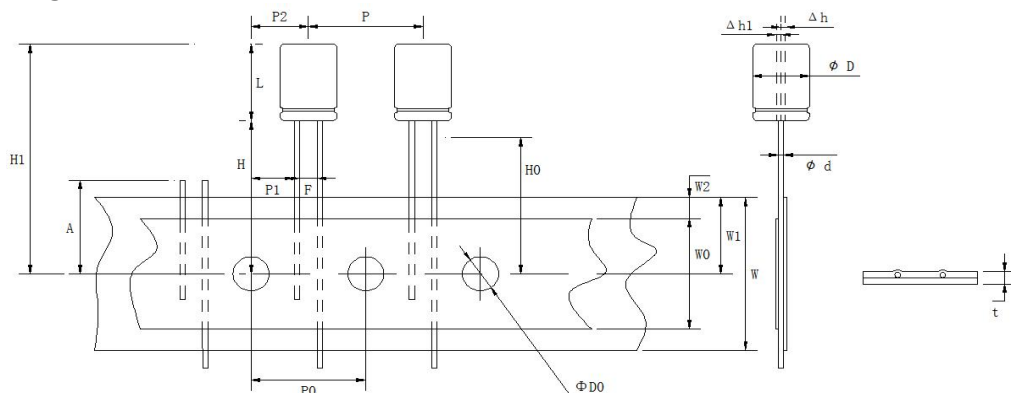
[ Fig. 4 (Diameter for \Phi 10 ) ]
