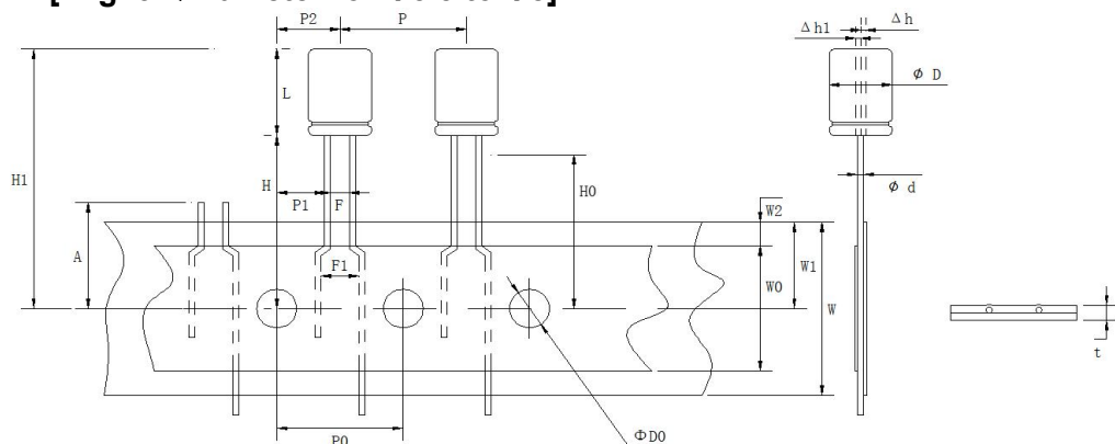
[ Fig. 3 (Diameter for \Phi 5.5 to \Phi 8 ) ]
