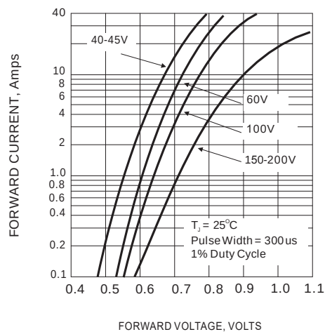
FIG.2-TYPICAL FORWARD CHARACTERISTICS
