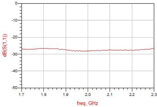
Figure 5. MHC21X03 Return Loss (S11)
