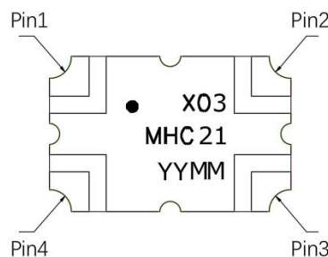
Figure 1. MHC21X03 (Top View)
