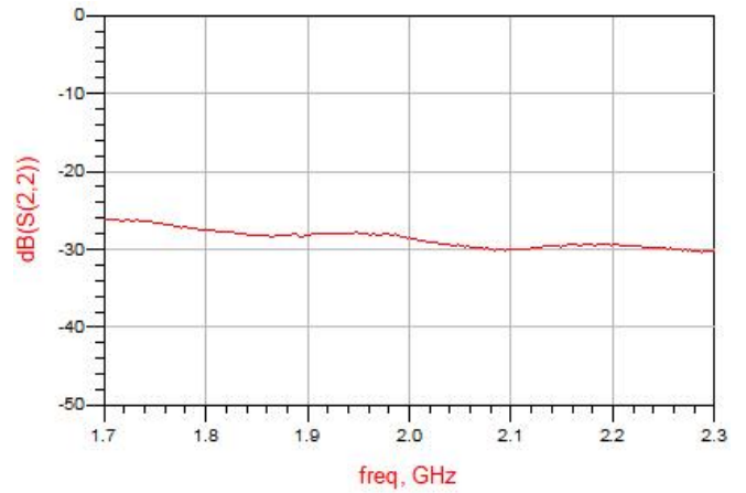
Figure 6. MHC21X03 Return Loss (S22)
