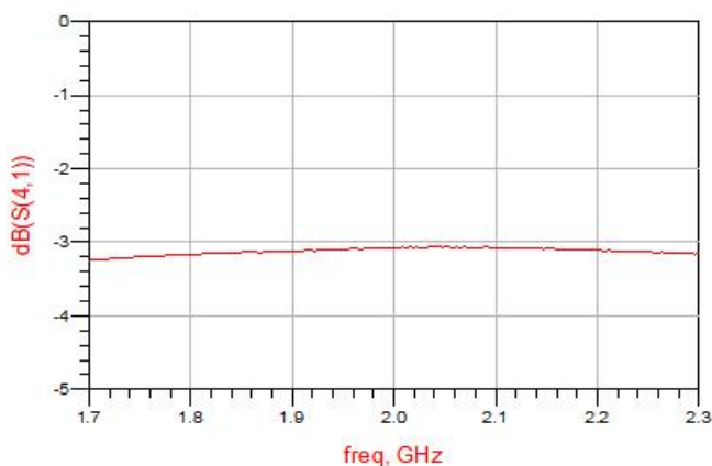
Figure 3. MHC21X03 Coupling
