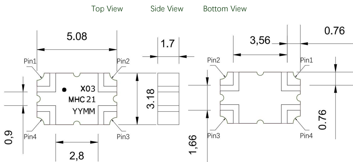
Figure 2. MHC21X03 Outline Drawing
