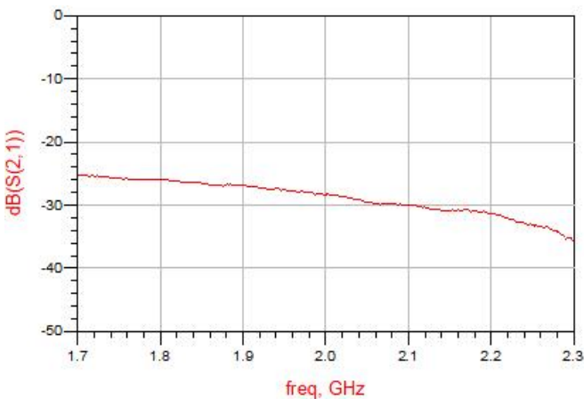
Figure 9. MHC21X03 Isolation
