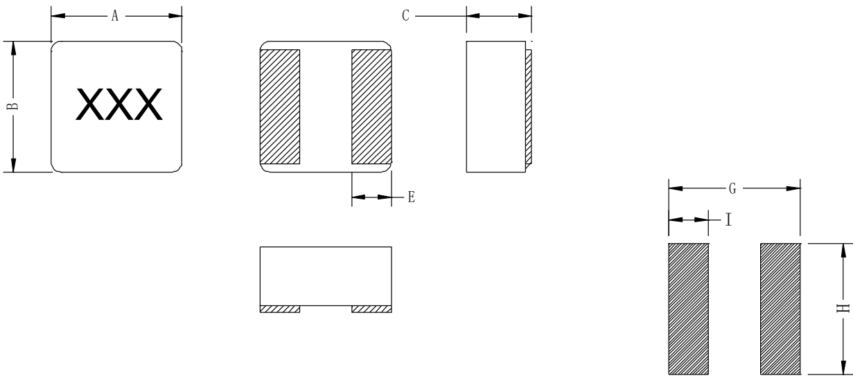
Product Exterior Schematic
