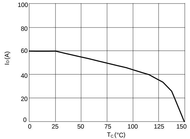
Figure 8: Current De-rating
