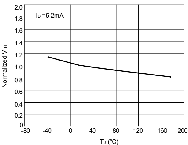
Figure 6: Normalized Threshold Voltage vs. Temperature
