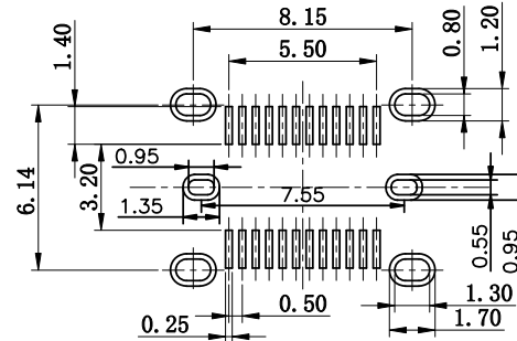
RECOMMENDED PCB LAYOUT(TOP VIEW) DEFAULT TOLERANCE: \pm 0.05
