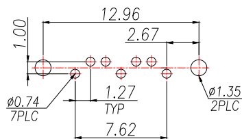
RECOMMEND PCB LAYOUT PCB TOLERANCE:±0.05
