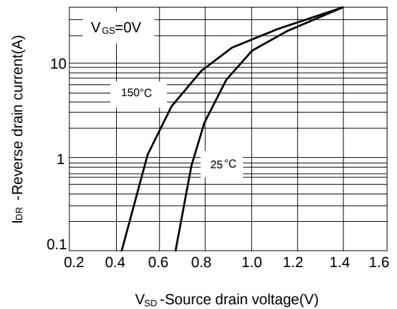
Figure 4: Body diode forward voltage
