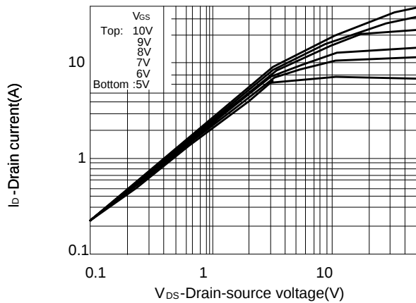
Figure 1: On-resistance characteristics
