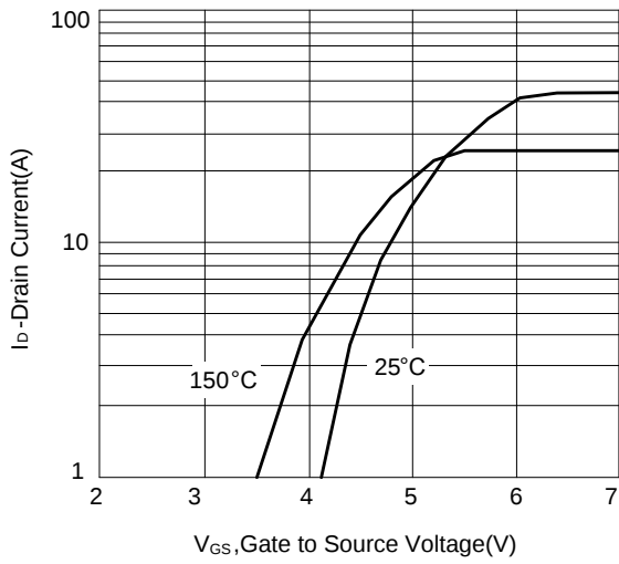
Figure 1: Transfer Characteristics
