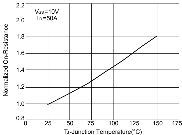
Figure 2: Rdson-Junction Temperature
