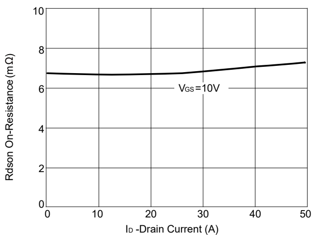
Figure 5: Rdson-Drain Current
