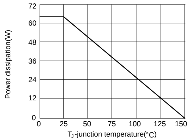
Figure 8: Power de-rating
