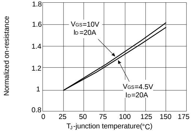
Figure 2: Rdson-junction temperature
