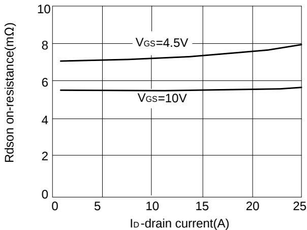
Figure 5: Rdson-drain current
