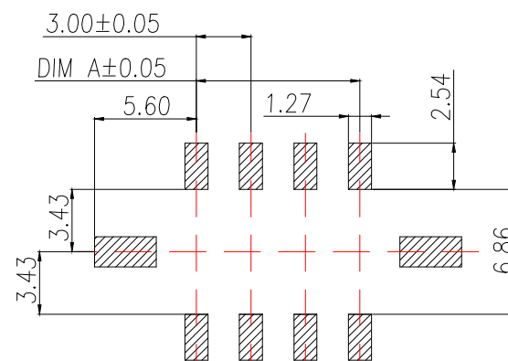
PCB.WELDING DRAWING (TOLERANCE:±0.05)
