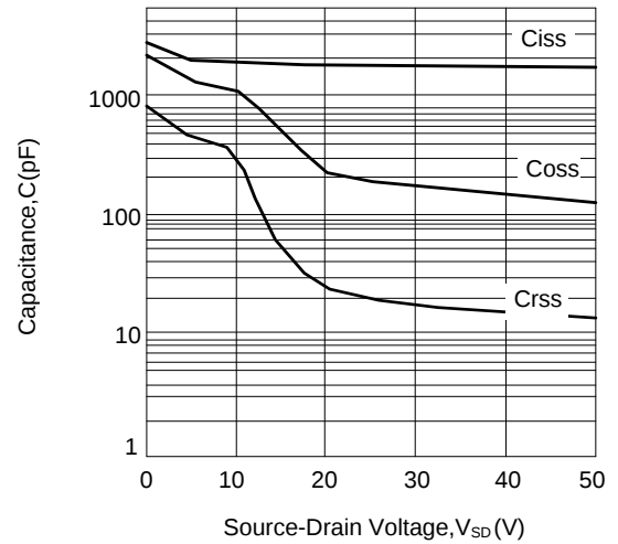
Figure 4: Capacitance Characteristics
