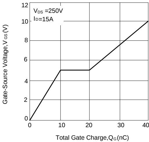
Figure 3: Gate Charge Characteristics
