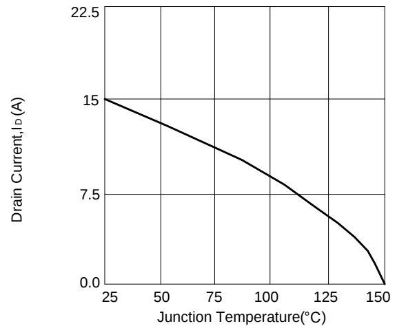
Figure 10: Drain-Current vs. Junction Temperature
