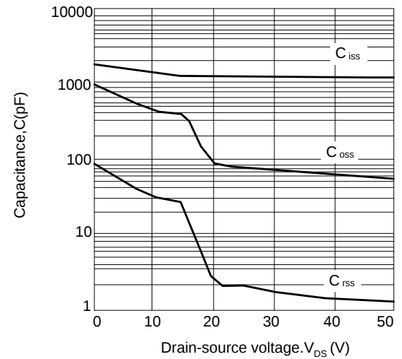
Figure 4: Capacitance characteristics
