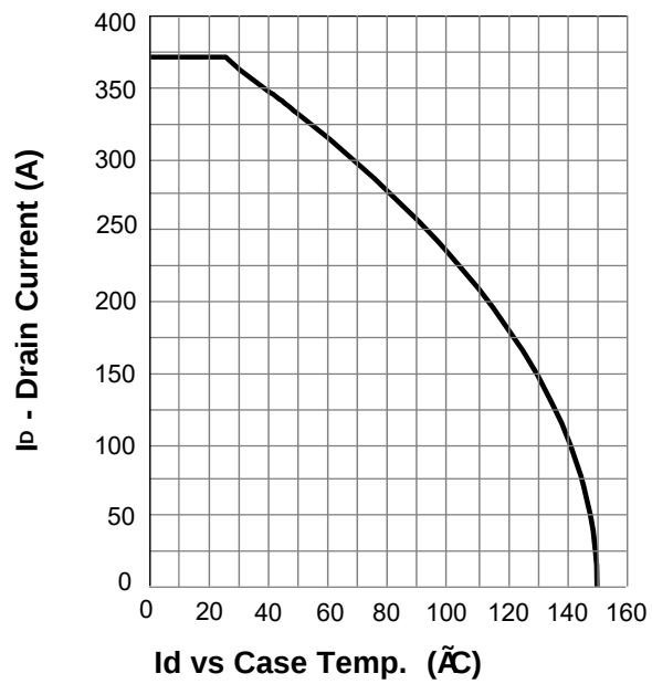
Current Capability
