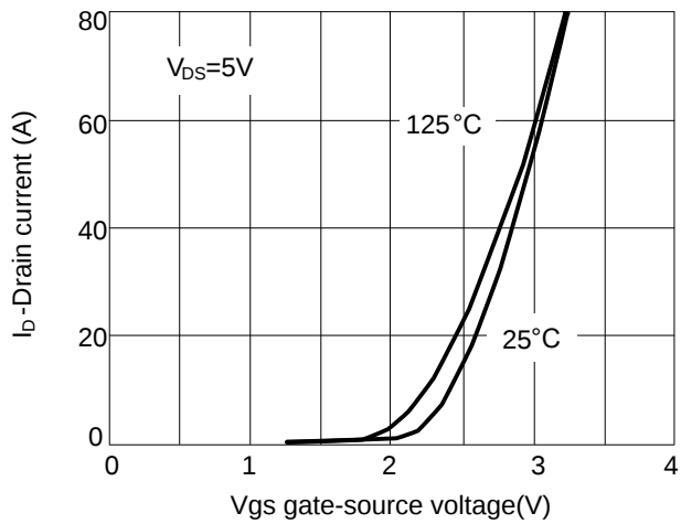
Figure 3 Transfer characteristics
