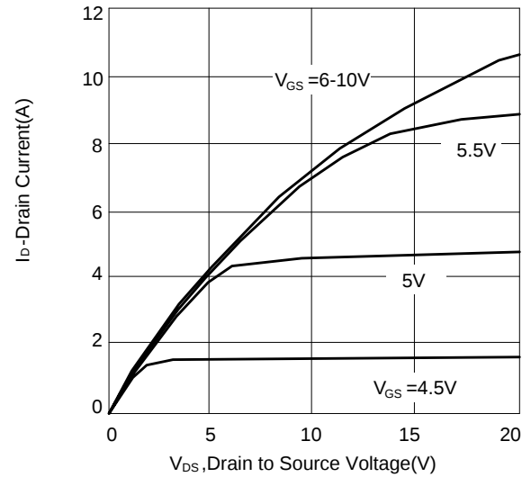
Figure 10: Output Characteristics
