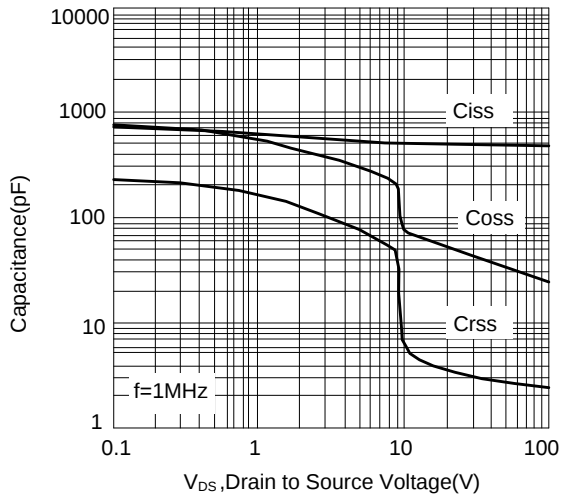
Figure 7: Capacitance vs Drain to Source Voltage
