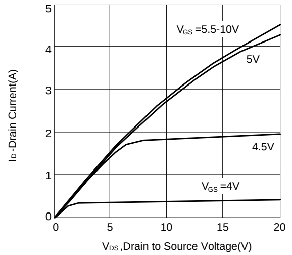
Figure 10: Output Characteristics
