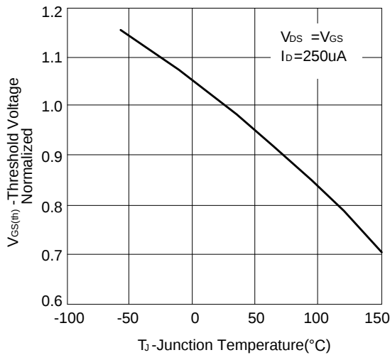
Figure 5: Threshold Voltage vs Junction Temperature
