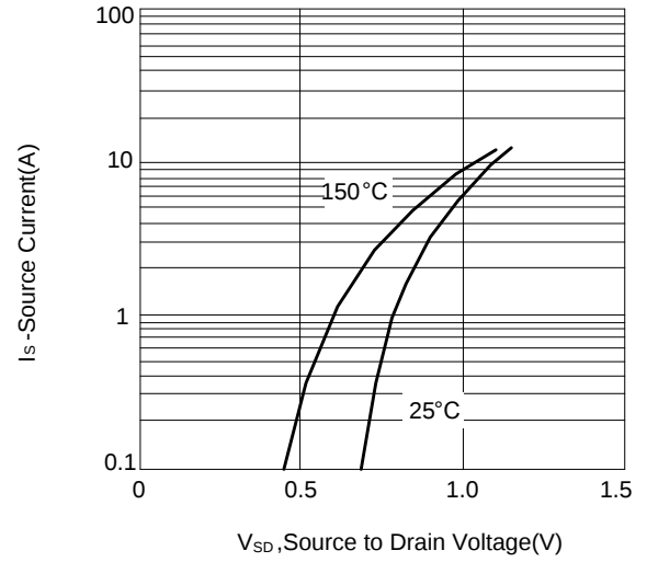
Figure 2: Body Diode Characteristics
