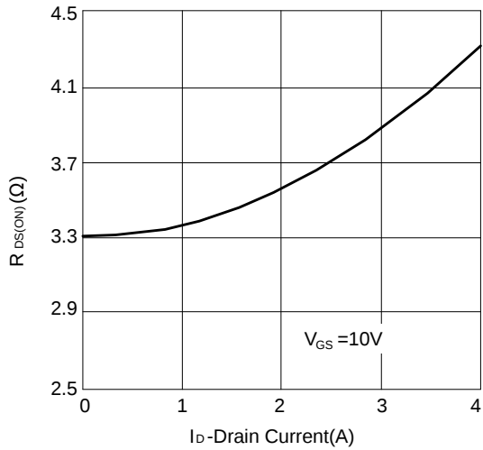
Figure 3: Drain to Source On-Resistance vs Drain Current
