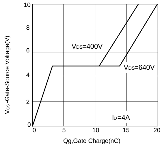
Figure 8: Gate Charge vs Gate to Source Voltage
