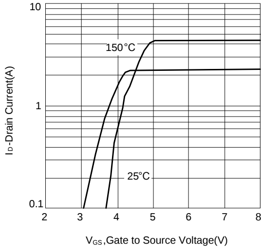
Figure 1: Transfer Characteristics
