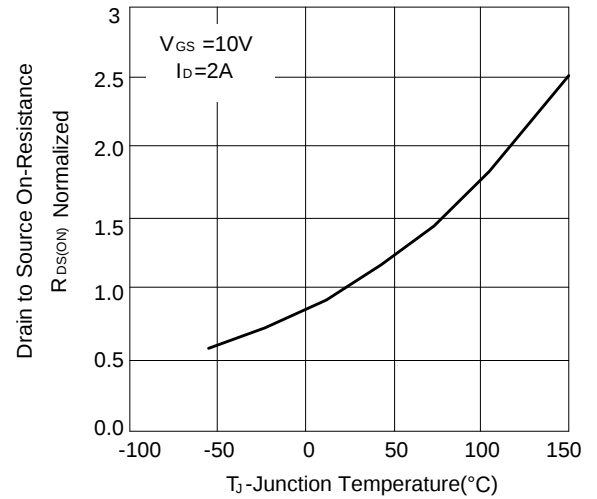
Figure 4: Drain to Source On-Resistance vs. Junction Temperature
