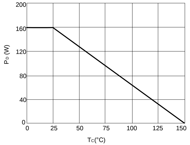
Figure 8: Power De-rating
