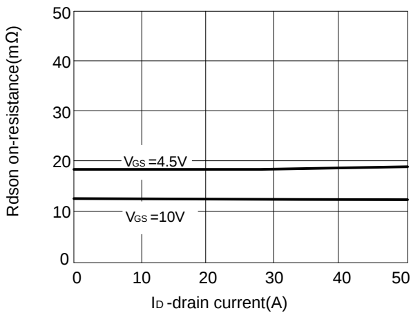
Figure 5: Rdson-drain current
