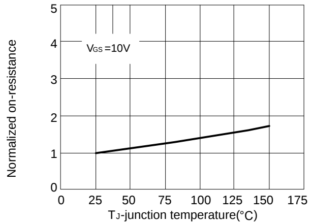
Figure 2: Rdson-junction temperature
