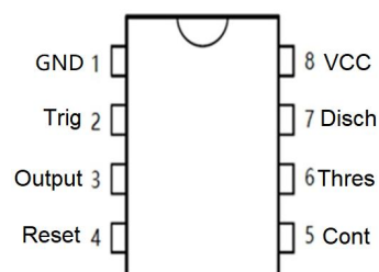
DIP-8/SOP-8/MSOP-8/TSSOP-8
