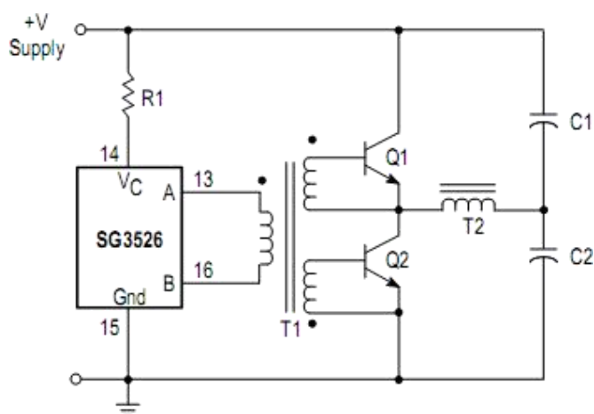
Half-Bridge Configuration
