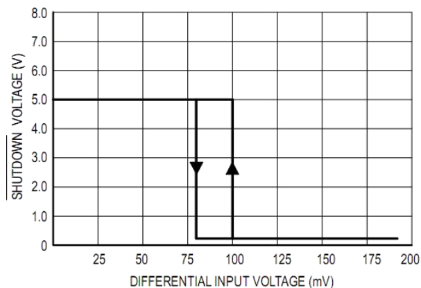
Current Limit Comparator Threshold
