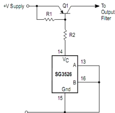
Single-Ended Configuration
