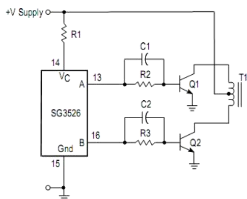
Push-Pull Configuration
