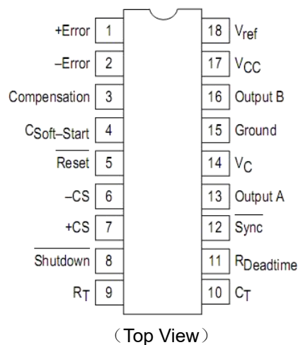
DIP-18/SOP-18W
