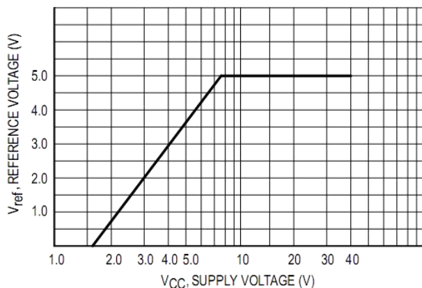
Reference Voltage as a Function Supply Votage
