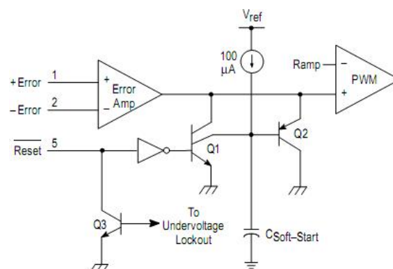
Soft-Start Circuitry
