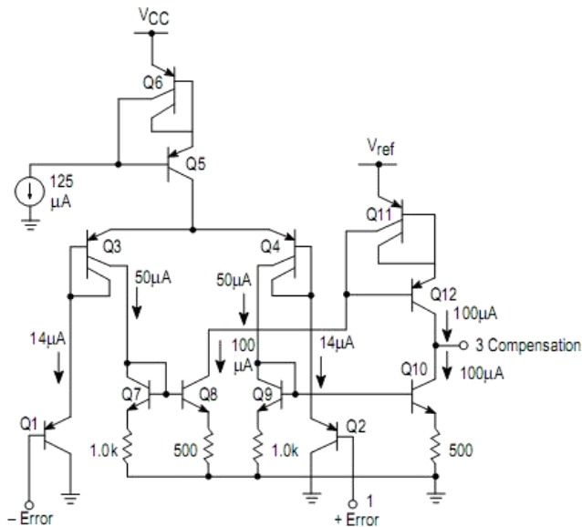
Error Amplifier
