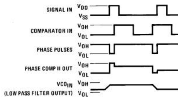
FIGURE 4. Typical Waveform Employing Phase Comparator II in Locked Condition
