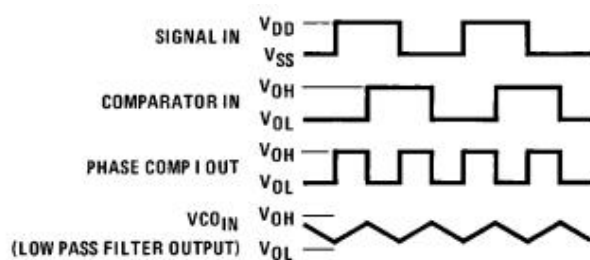
FIGURE 3. Typical Waveform Employing Phase Comparator I in Locked Condition
