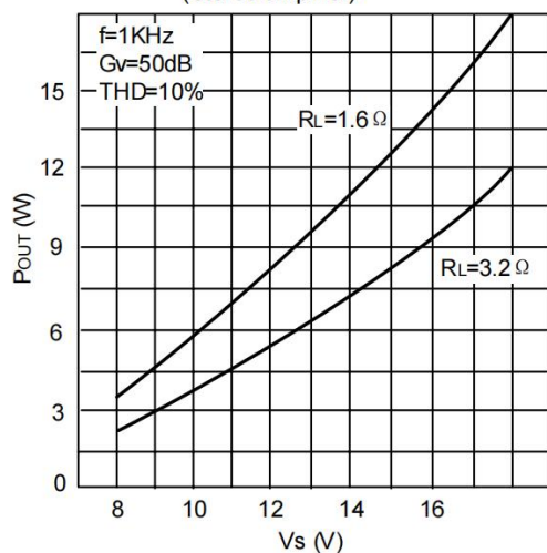
Figure 14. Output Power versus Supply Voltage (Stereo amplifier)
