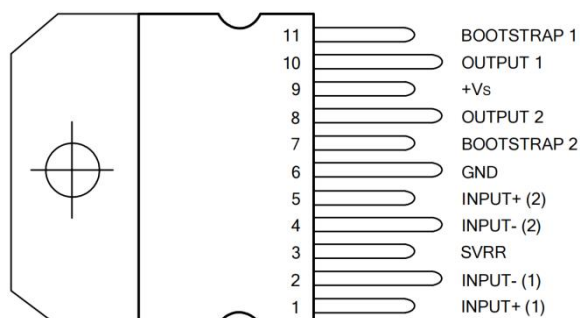
ZIP-11/Multiwatt11
