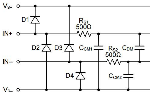
Figure 1. Input EMI Filter and Clamp Circuit
