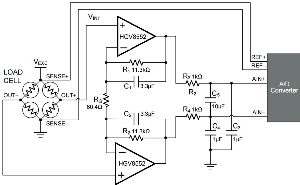
Figure 12. Precision Weigh Scale Measurement System
