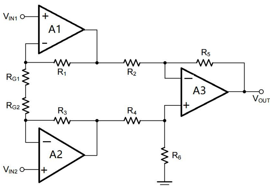
Figure 10. Discrete 3-Op-amp Instrumentation Amplifier
