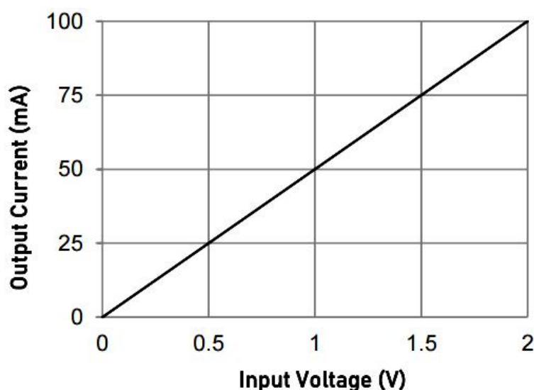
Figure 9. Measured Transfer Function for High-Side V-I Converter
