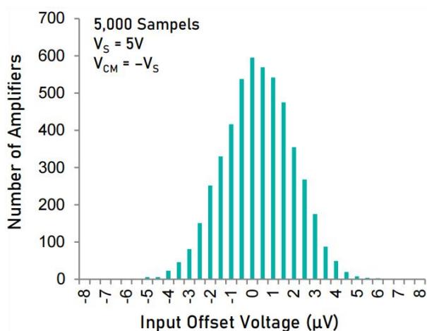
Input Offset Voltage Production Distribution.
