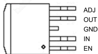
TO-252-4
