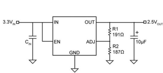
IFX1963 Adjustable Output Regulator
