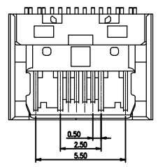
SECTION B-B SCALE 1:1
