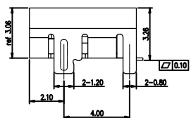
SECTION B-B SCALE 1:1
