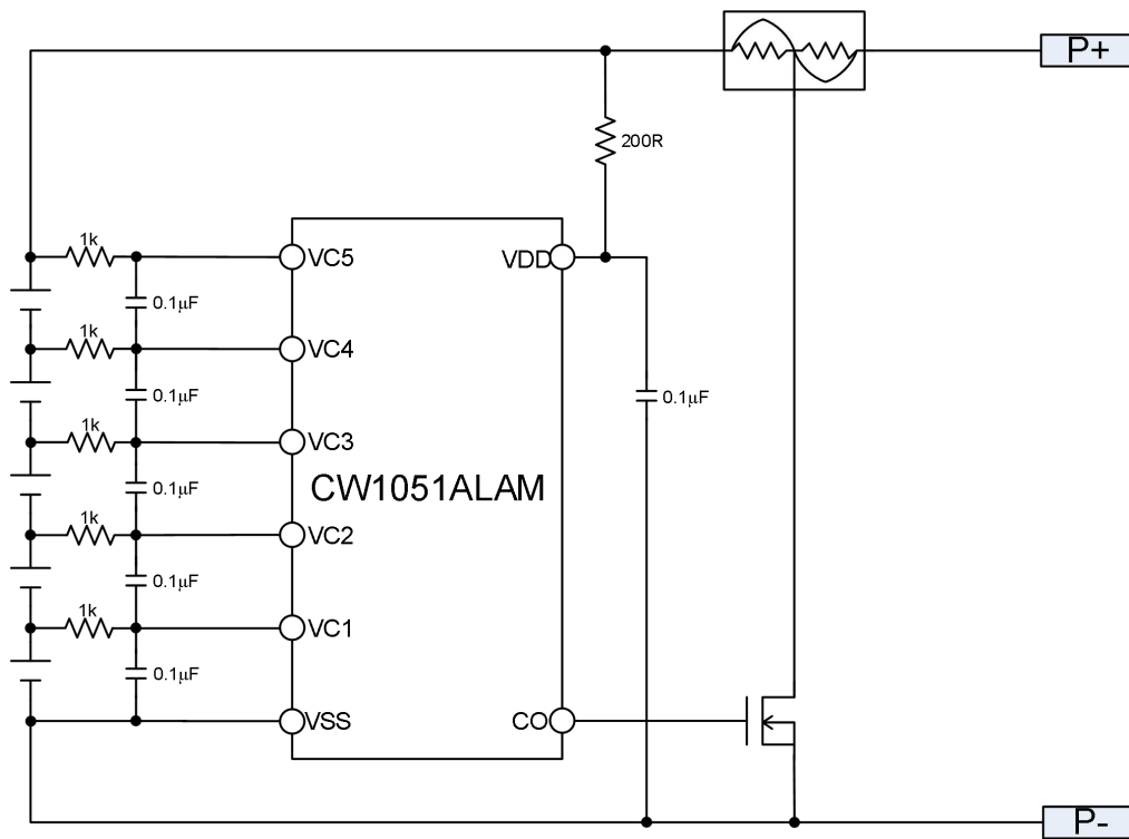
Reference Schematic for 5 cells
