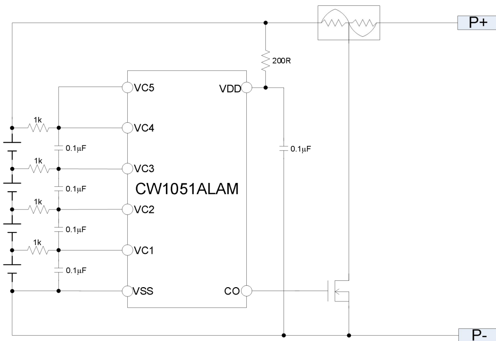
Reference Schematic for 4 cells(connect high side cell)
